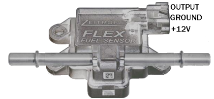
Flow Through Flex Fuel Sensor Pinout
